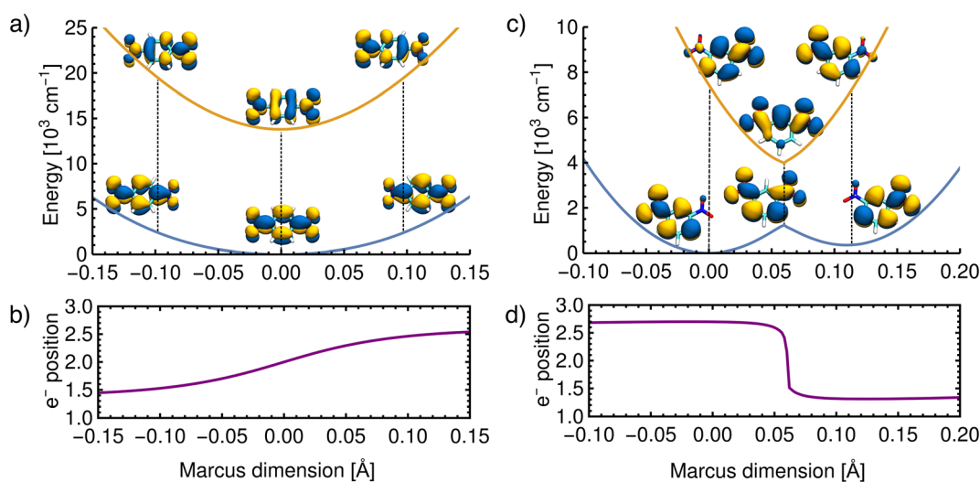
Fig. 6 Reconstructed potential energy curves from geometries displaced in the direction of the Marcus dimension using the electronic energies. (a) Results for p -DNB •- in ACN. The scan was performed with a step size of 0.005 Å. (b) The electron position for p -DNB •- . (c) Results for m -DNB •- in ACN. The scan was performed with a step size of 0.002 Å. (d) The electron position for m -DNB •- . The change of the electron position in the ground and excited states is illustrated in the upper panels using natural transition orbitals and quantified in the lower panels according to eqn (3).
