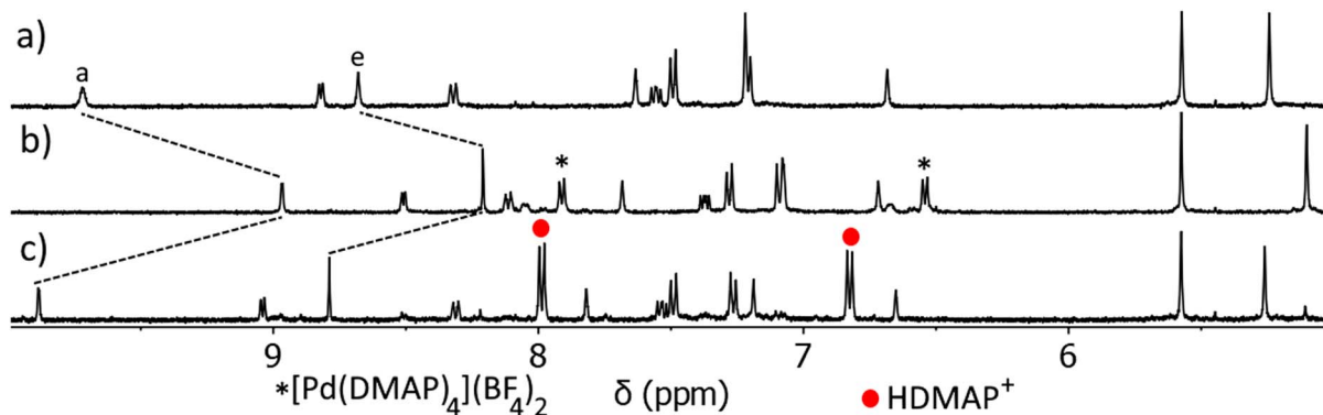
Fig. 6 Stacked partial ^1\text{H} NMR spectra (400 MHz, \text{CD}_3\text{CN} , 298 K) of (a) \text{C} \llcorner \text{MsO}^- at a 1 : 1 ratio ([C] = 1.00 mM), (b) [\text{Pt}(\text{L})_4](\text{BF}_4)_2 open complex after the addition of DMAP (4 eq.), (c) restored \text{C} \llcorner \text{MsO}^- host-guest adduct after addition of \text{MsOH} (4.1 eq.).
