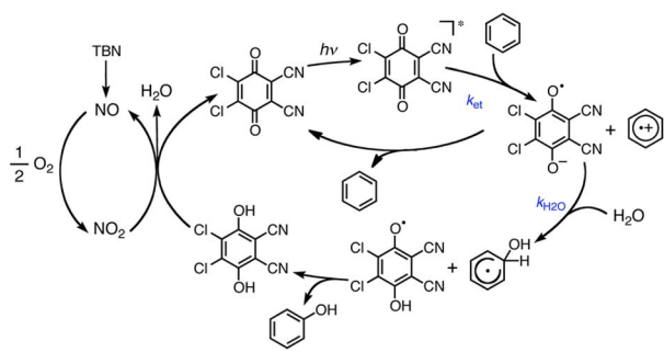
Scheme 7 A mechanism for photohydroxylation of benzene by dioxygen with DDQ used as a photoredox catalyst in the presence of TBN and H_2O in MeCN under photoirradiation. Reprinted from ref. 44 with permission from American Chemical Society (Copyright 2013).
