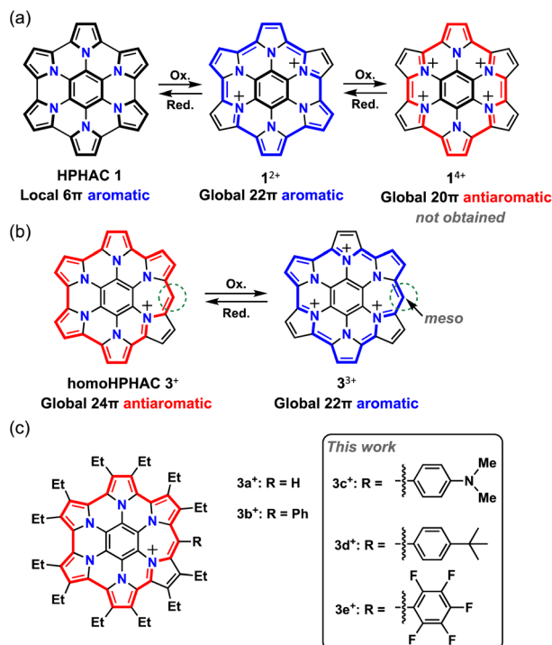
Fig. 1 (a) Chemical structures of HPHAC 1 and its cationic species. (b) Resonance structures of antiaromatic homoHPHAC 3^+ and aromatic 3^{3+} . (c) HomoHPHAC 3^a – 3^e with the various substituents studied in this work.
