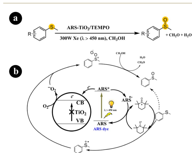
Scheme 5 (a) The reaction conditions for this process include specific parameters such as the type of catalyst (ARS-sensitized TiO 2 ), the presence of a co-catalyst (TEMPO), the use of visible light as the energy source, and the involvement of molecular oxygen (aerobic conditions). (b) One potential mechanistic route for the visible light photocatalytic aerobic oxidation of thioanisole involves ARS-sensitized TiO 2 and TEMPO. Reproduced with permission from ref. 40. Copyright 2016, John Wiley and Sons.
