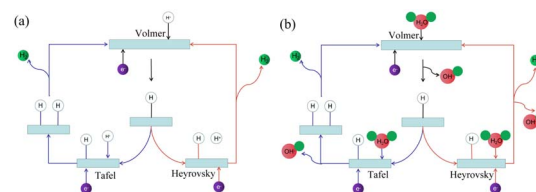
Fig. 1 Hydrogen evolution reaction mechanism. (a) Schematic diagram of hydrogen evolution reaction in acidic solution. (b) Schematic diagram of hydrogen evolution reaction in alkaline solution.
