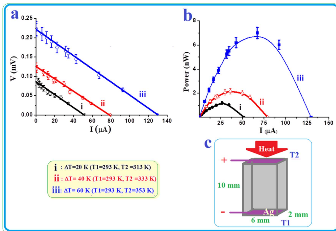
Fig. 7 Above and near RT thermoelectric power characteristics of a single leg TE module made of the Gr-NDs nanocomposite in compact rectangular form (of 2 × 6 × 10 mm) at different \Delta T values. (a) Open and closed-circuit values of V vs. I , (b) power output vs. I , and (c) dimensions of the used single-leg using rectangle-shape module.
