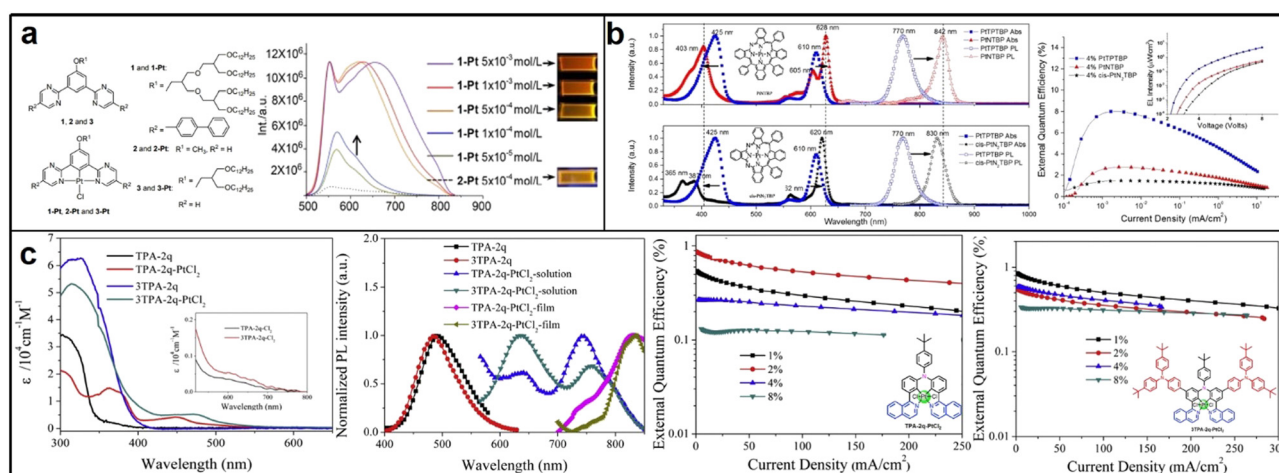
Fig. 6 (a) N + C + N + -type tridentate ligand-based Pt(II) complexes; reproduced with permission from ref. 59. Copyright 2017 Chinese Journal of Organic Chemistry (b) PtNTBP and cis -PtN 2 TBP; reproduced with permission from ref. 61. Copyright 2016 Applied Physics Letters . (c) TPA-2q-PtCl 2 and 3TPA-2q-PtCl 2 . Reproduced with permission from ref. 62. Copyright 2017 Dyes and Pigments .
