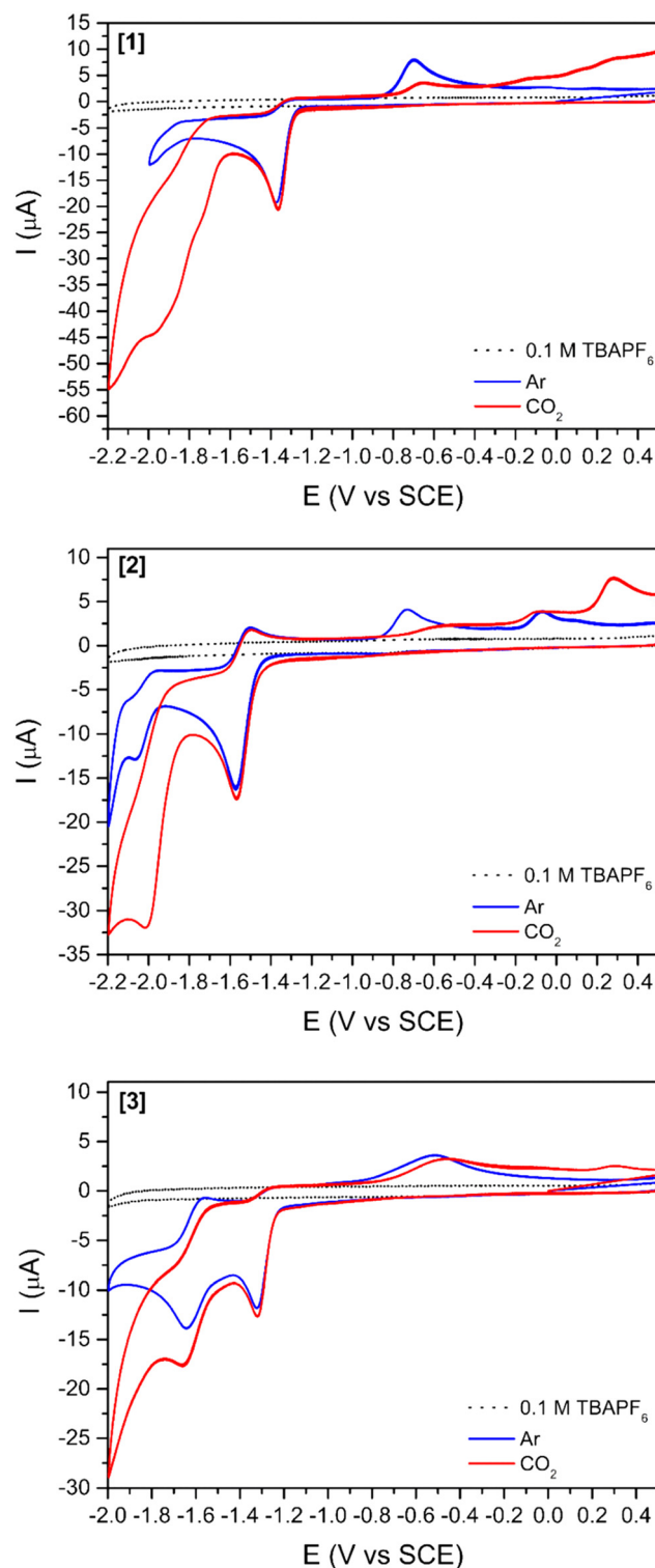
Fig. 2 Cyclic voltammograms of complexes [1], [2], and [3] (1 mM) in DMF, argon, or carbon dioxide saturated solutions using TBAPF 6 as supporting electrolyte (0.1 M) at 100 \text{ mV s}^{-1} . Glassy carbon (3 mm diameter) was used as working, platinum wire as counter and SCE as reference electrodes.
