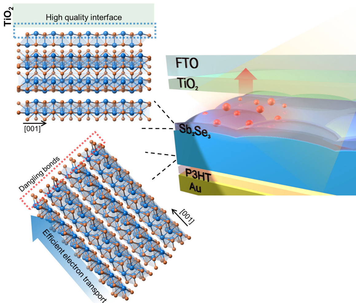
Fig. 6 Schematic illustration of the proposed novel bilayer Sb 2 Se 3 configuration that can effectively transport the charge carriers without recombination and also form a high quality interface with the TiO 2 layer.
