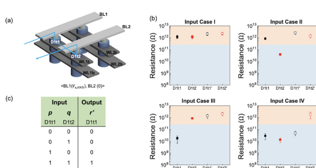
Fig. 5 Experimental demonstration of the AND logic gate between D_{11\text{t}} and D_{12\text{t}} memristors in the BLC. (a) The bias configuration in the schematic diagram of the vertical CBA, where V_{a,\text{AND}} = +9 V. (b) The results of the AND logic operation in D_{11\text{t}} for each input case. A resistance lower than 250 \text{ G}\Omega is encoded to the "1" state and (c) its truth table of the logic gate.
