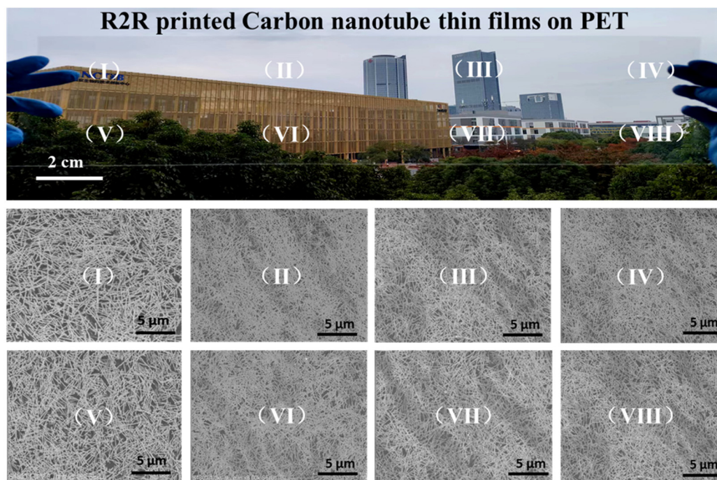
Fig. 3 SEM images of sc-SWCNT networks in different areas of 8 cm \times 14 cm sc-SWCNT thin films on a PET substrate.
