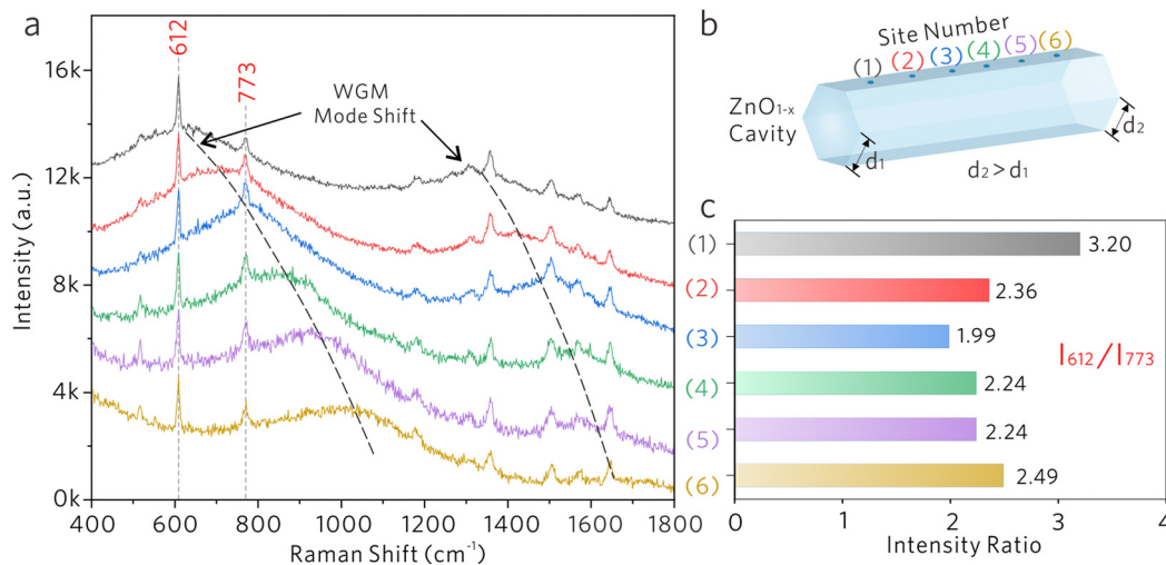
Fig. 6 WGM cavity sensing mechanisms: optical resonance coupling. (a) Raman spectra collected from a \text{ZnO}_{1-x} cavity ( d \approx 2 \mu\text{m} ) with a side length gradient. (b) Schematics of the \text{ZnO}_{1-x} cavity with side length gradient. (c) The Raman intensity ratio columns of I_{612}/I_{773} from different sites.
