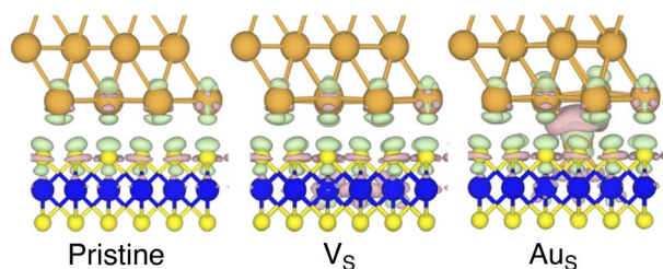
Fig. 4 Electron density difference (EDD) maps of the pristine, V_{\text{S}} and Au 5 interfaces in the vicinity of the contact area. Green colour corresponds to electron loss, whereas mauve colour to electron enrichment. The isovalue was set to 0.002 \text{ eV } \text{\AA}^{-3} .
