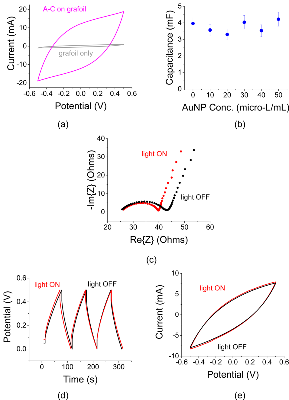
Fig. 3 (a) C–V traces for AC coated (pink curve) and uncoated (gray curve) current collectors made of bare grafoil. The scan rate was large, 100 \text{ mV s}^{-1} . (b) Varying concentration of AuNPs on grafoil only electrodes exhibited little capacitance variations. The concentration of the AuNPs is referenced to the solvent: 1 mL of acetone, hence \mu\text{L} of Au suspension to mL of solvent. The electrolyte was 1 M NaCl. (c) EIS curves under a continuous 75 W white-light exposure for the colloid embedded sample on ITO transparent substrates. (d) Corresponding C–D traces at I_0 = 1 mA (charge density, J_0 = 0.62 \text{ mA cm}^{-2} ) and (e) C–V traces at a scan rate of 100 \text{ mV s}^{-1} revealed small light induced effects.
