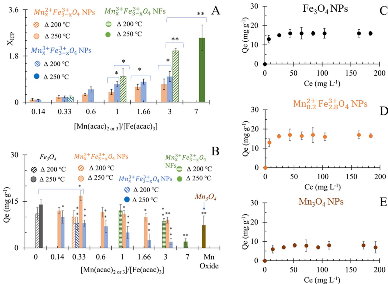
Fig. 5 (A) Elemental analysis of \text{Mn}_x\text{Fe}_{3-x}\text{O}_4 NS that were prepared at 200 °C and 250 °C. * P < 0.05 and ** P < 0.01 in comparison to \text{Mn}^{3+}\text{Fe}_{3-x}\text{O}_4 NPs of similar precursor ratios; (B) adsorption capacity of NPs for \text{Cr}^{6+} , * P < 0.05 and ** P < 0.01 in comparison to \text{Fe}_3\text{O}_4 NPs; (C)–(E) adsorption isotherm of \text{Ce}^{6+} by \text{Fe}_3\text{O}_4 , \text{Mn}_{0.2}^{2+}\text{Fe}_{2.8}^{3+}\text{O}_4 and \text{Mn}_3\text{O}_4 NPs respectively.
