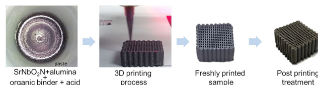
Fig. 2 (left) SrNbO 2 N-containing printing ink prepared by mixing SrNbO 2 N/Al 2 O 3 powder, organic binder and acid solution to obtain a printable viscosity; resulting 3D printed monolith freshly printed, dried and thermally treated (viewed from left to right).
