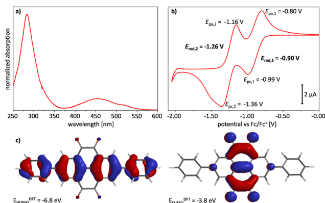
Fig. 2 (a) UV/Vis spectrum of compound 2 measured in CH 2 Cl 2 at rt (1 \mu\text{mol L}^{-1} ). (b) Cyclic voltammogram of model compound 2 (CH 2 Cl 2 , n Bu 4 NPF 6 (0.1 M), measured at rt with Pt-working electrode and (Fc/Fc + ) as internal reference, scanning velocity: 100 mV s −1 ). (c) DFT model (B3LYP: 6-311++G**) of compound 2 (tert-butyl groups omitted).
