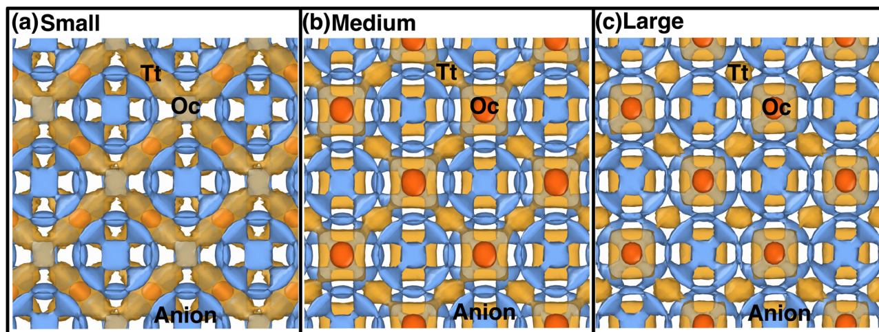
Fig. 8 Isosurface density plots of the cation (isovalues of 2 \times 10^4 \text{ \AA}^{-3} (orange) and 6 \times 10^5 \text{ \AA}^{-3} (red)) and H-atom for MCB_{11}H_{12} ( M = small, medium, and large) in a 2 \times 2 supercell obtained using OVITO 70 software at 475 K from NVE-MD simulations. (a) Isovalue 7.5 \times 10^{-5} \text{ \AA}^{-3} (blue) for small-sized cation. (b) Isovalue 7.5 \times 10^{-5} \text{ \AA}^{-3} (blue) for medium-sized cation. (c) Isovalue 7.5 \times 10^{-5} \text{ \AA}^{-3} (blue) for large-sized cation. Tt- and Oc-sites formed by anions are marked. We choose different H isovalues for different sizes of cation cases for better visualization.
