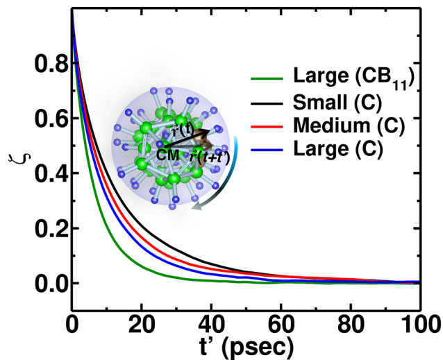
Fig. 7 Angular autocorrelation function \zeta(t') of the C and anion from NVE-MD simulation at 475 K for MCB_{11}H_{12} ( M = small, medium, and large) system. CB_{11} means that the averaging is performed over twelve atoms (one C and eleven B atoms), whereas C indicates the averaging over only C. The function \zeta(t') of the anion ( CB_{11} ) for a large-sized cation system is also included for the comparison.
