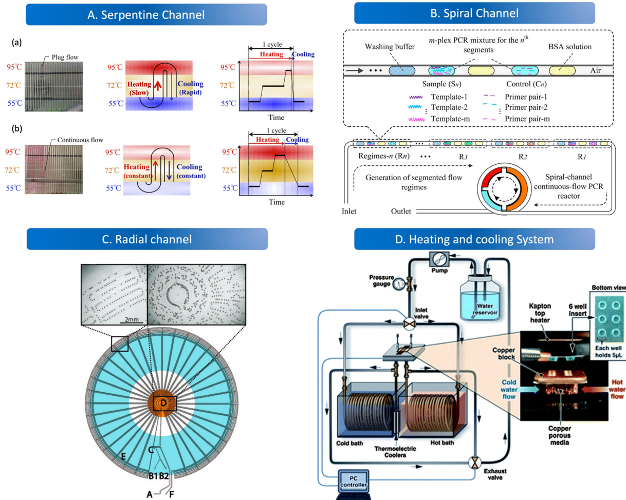
Fig. 4 Features of the thermal cycle. A. Serpentine channel. (a) Plug flow-based thermal cycling technique presented by using a temperature gradient between 95 °C and 55 °C; (b) continuous flow-based thermal cycling. Copyright 2014 by MDPI. 97 B. Spiral channel. Illustration of design principle of spiral-channel segmented continuous-flow multiplex PCR amplification. Copyright 2014 by Elsevier. 102 C. Radial channel. The device contains an oil inlet (A) that joins two aqueous inlet channels (B1 and B2) to form droplets at a T-junction (C). The droplets pass through the inner circles (500 μm wide channels) in the hot zone (D) to ensure initial denaturation of the template and travel to the periphery in 200 μm wide channels where primer annealing and template extension occur (E). The droplets then flow back to the center, where the DNA is denatured and a new cycle begins. Finally, the droplets exit the device after 34 cycles (F). Copyright 2009 by ACS. 103 D. Heating and cooling system. System schematic with an expanded view in the insert, wells and Kapton heater. Copyright 2011 by RSC. 105
