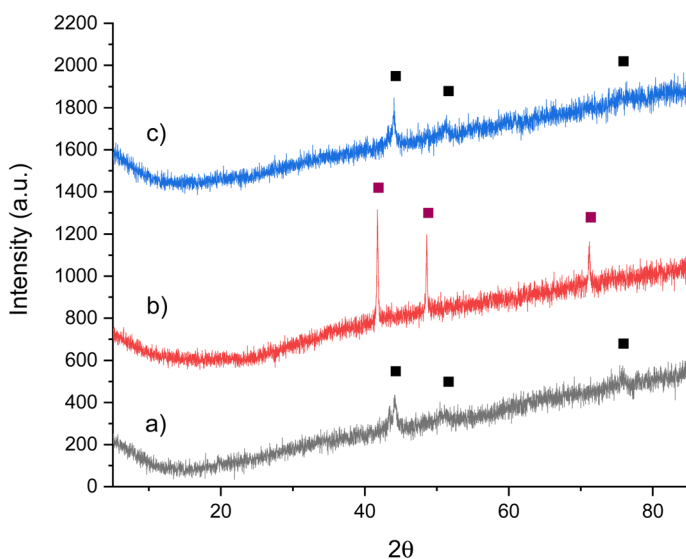
Fig. 4 XRD patterns of \text{Co}_3\text{CuN} : (a) post 1st cycle with 3 : 1 \text{ H}_2/\text{N}_2 at 300^\circ\text{C} , (b) pre 2nd cycle and (c) post 2nd cycle with 3 : 1 \text{ H}_2/\text{N}_2 at 300^\circ\text{C} . (■) \text{Co}_3\text{CuN} and (■) \text{Co}_3\text{Cu} .
