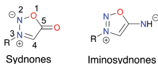
Fig. 1 General structure of sydnones and iminosydnonones.
