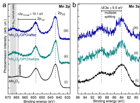
Fig. 5 XPS spectra of (a) Mn- 2p and (b) Mn- 3s regions of the \text{Mn}_2\text{O}_3 electrodes before (ii) and after (iii) the electrochemical performance. The spectra of the Mn oxide prior to be mixed with the graphite powder is provided as reference (i). The relative energy position of the 2p_{1/2} satellite and the constant magnitude of multiplet splitting in the 3s component supports the existence of a stable \text{Mn}^{3+} oxide.
