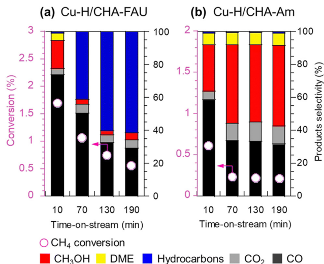
Fig. 14 Catalytic performance of (a) Cu-H/CHA-FAU and (b) Cu-H/CHA-Am in the partial oxidation of methane. Reaction conditions: 100 mg catalyst; P_{\text{CH}_4} : P_{\text{N}_2\text{O}} : P_{\text{H}_2\text{O}} : P_{\text{Ar}} = 0.4 : 0.4 : 0.08 : \text{balance} ; total pressure 0.1 MPa; \text{SV} = 15\,000 \text{ mL h}^{-1} \text{ g}_{\text{cat}}^{-1} ; W/F = 3.7 \text{ g}_{\text{cat}} \text{ h mol}_{\text{CH}_4}^{-1} ; 623 K. Reprinted from ref. 63 with permission from Royal Society of Chemistry, copyright 2023.
