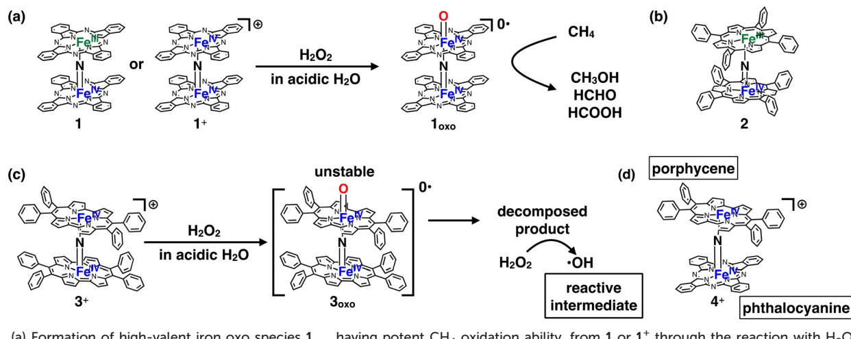
Fig. 1 (a) Formation of high-valent iron oxo species 1_{\text{oxo}} having potent \text{CH}_4 oxidation ability, from 1 or 1^+ through the reaction with \text{H}_2\text{O}_2 . (b) A \mu -nitrido-bridged iron porphyrin dimer ( 2 ) showing potent \text{CH}_4 oxidation ability. (c) Structure of a monocationic \mu -nitrido-bridged iron porphycene dimer ( 3^+ ) and its proposed \text{CH}_4 oxidation mechanism. (d) A monocationic \mu -nitrido-bridged heterodimer of an iron porphycene and an iron phthalocyanine ( 4^+ ) synthesized in this work.
