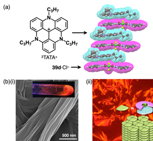
Fig. 27 (a) Single-crystal X-ray structure of ^3\text{TATA}^+ \cdot 39\text{d} \cdot \text{Cl}^- (redrawn from a cif file: 745780) and (b) (i) photograph and SEM of the supramolecular gel and (ii) POM and packing model of the liquid crystal mesophase of ^3\text{TATA}^+ \cdot 39\text{e} \cdot \text{Cl}^- (redrawn from ref. 7. Copyright 2010 Wiley).
