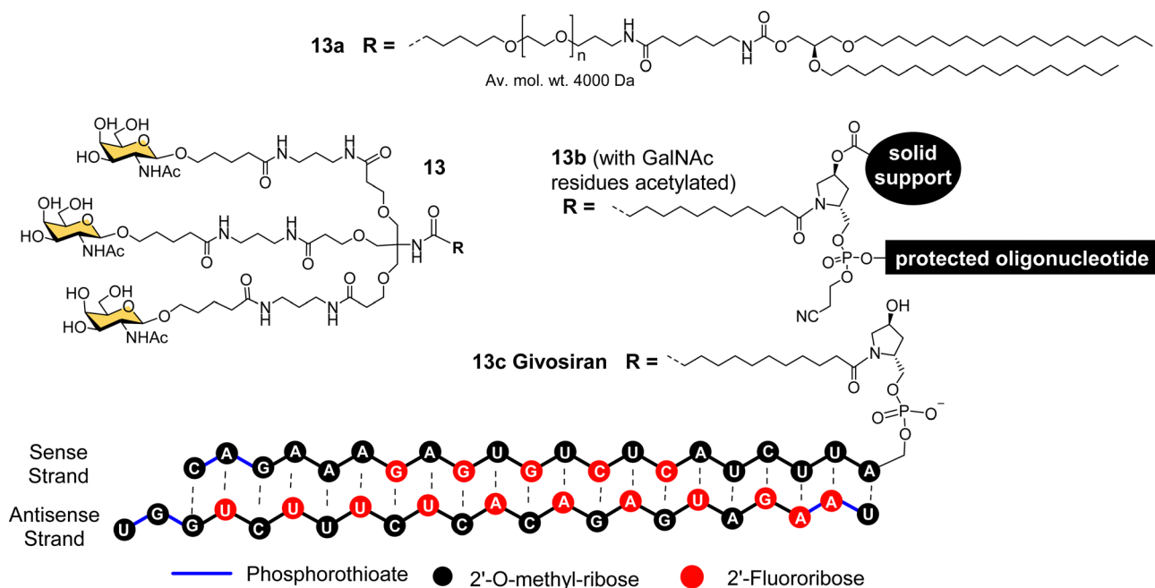
Fig. 6 Chemical structure of triantennary GalNAc ligand 13 developed by Alnylam Pharmaceuticals for lipid conjugates ( 13a ), solid-supported oligonucleotide synthesis ( 13b ) and siRNA drug Givosiran ( 13c ).
