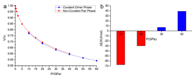
Fig. 8 Comparison between the phases containing non-covalent \pi -pairs and covalent \sigma -dimers of the (\text{TTF-BTD})_2\text{I}_3 crystal structure. (a) Variation of the normalized unit cell volume with pressure; (b) difference of "pseudo-enthalpy" ( E_{\text{el}} + \text{PV} ) between the two phases at selected pressures. Negative values indicate that the non-covalent \pi -pair is more stable, while positive values indicate that the covalent \sigma -dimer is favoured.
