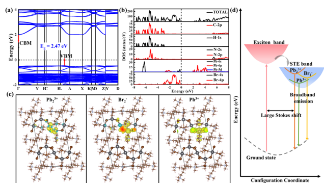
Fig. 4 (a) Calculated electronic band structures and (b) DOS of (HM)Pb 2 Br 6 . (c) Calculated charge density for (HM)Pb 2 Br 6 (Pb 2 3+ STEs, Br 2 - and Pb 3 + STLHs holes) upon crystal lattice perturbation via the Pb–Pb, Br–Br and Pb–Br distances shortening. (d) Configuration coordinate diagram illustrating the luminescence mechanism.
