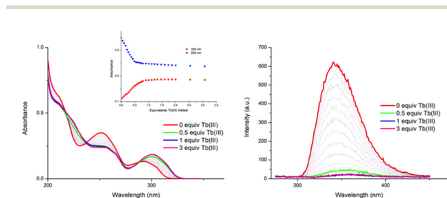
Fig. 2 The overall changes in the (left) UV-visible absorption spectra and (right) fluorescence emission spectra ( \lambda_{exc} = 260 nm) upon titrating 1 ( 1 \times 10^{-5} M) against Tb(CF_3SO_3)_3 (0 \rightarrow 3 equiv.) in CH_3CN at 22 °C. Inset: The binding isotherms of absorbance at \lambda = 300 and 250 nm, respectively.
