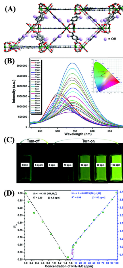
Fig. 2 (A) 3D framework structure of LMOF 3 . (B) Relative changes in fluorescence intensity of 3 upon increasing aqueous NH 3 concentration from 0 to 100 ppm in DMA medium. (C) Photographs for the turn-off and turn-on fluorescence behavior triggered by aqueous NH 3 . (D) Linear relationship between the observed efficiency of fluorescence changes and the aqueous NH 3 concentration was recorded in DMA. Reprinted with permission from ref. 48. Copyright 2018 Royal Society of Chemistry.
