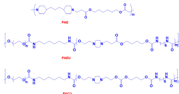
Fig. 2 Chemical structure of pH-responsive cationic polymers.
