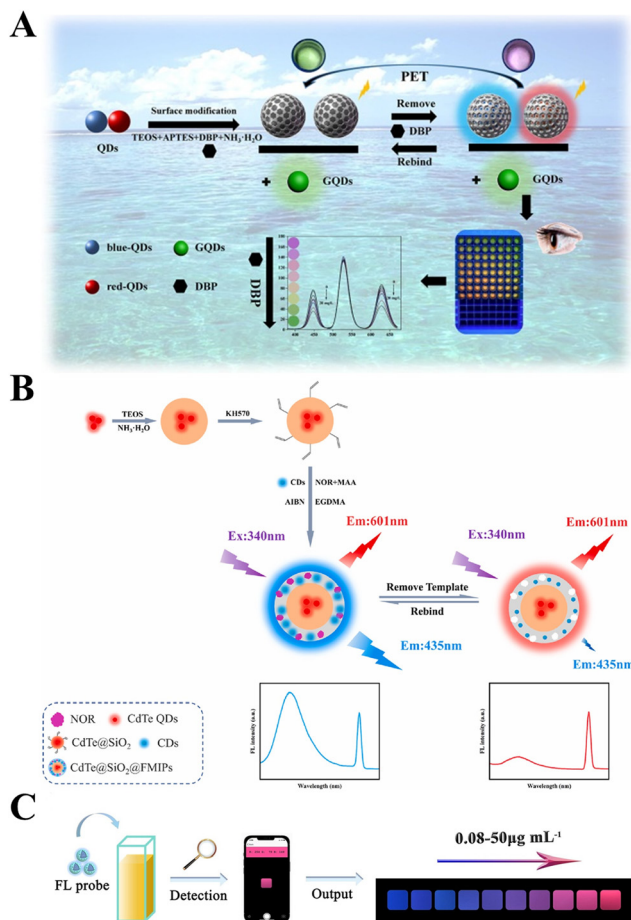
Fig. 4 Schematic illustration of the MI-RFL sensors for the detection of new pollutants. (A) Sensor construction and detection process for DBP. 98 (B) Preparative strategy of CdTe@SiO 2 @FMIPs for the detection of NOR. 97 (C) The developed smartphone-integrated sensing platform to detect OTC. 80
