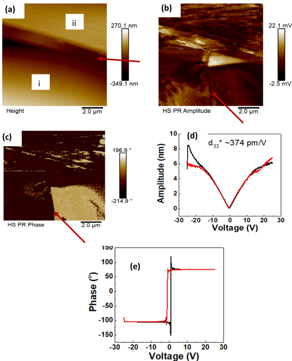
Fig. 4 Piezoresponse Force Microscopy (PFM) studies on the BT-1500 pellet – (a) Surface topography, where the arrow indicates the grain boundary; parts of two grains are indicated with numbers. (b) and (c) PFM amplitude and phase images at zero bias voltage, where arrows indicate the domain wall boundary; (d) and (e) PFM amplitude and phase under different bias voltage. Converse piezoelectric coefficient ( d_{33}^* ) determined from the slope at the linear region in (d).
