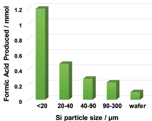
Fig. 4 Effect of silicon particle size on formic acid yield from the reaction system of \text{CO}_2 , \text{H}_2\text{O} , and powdered silicon wafer catalysed by \text{TBAF}\cdot\text{3H}_2\text{O} . Reaction conditions: powdered silicon wafer (5 mmol), \text{CO}_2 (0.1 MPa, balloon), \text{H}_2\text{O} (10 mmol), \text{TBAF}\cdot\text{3H}_2\text{O} (0.05 mmol), DMSO (2 mL), 95 ^\circ\text{C} , 24 h. Yield was determined through internal standard technique of ^1\text{H} NMR with \text{CDCl}_3 as the solvent and 1,3,5-triisopropylbenzene as the internal standard.
