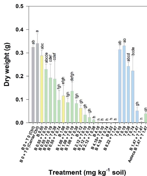
Fig. 3 Dry weight of Brassica napus following a 14 day exposure to bentazone (B) and terbuthylazine (T), singly and in mixture, or to Asteca® Mays diluted to the same concentration tested in one of the mixture treatments. The bars stand for the average of three replicates and the error bars for the respective standard error. Significant differences are presented for each treatment (Tukey's test, p < 0.05 ) using lowercase letters.
