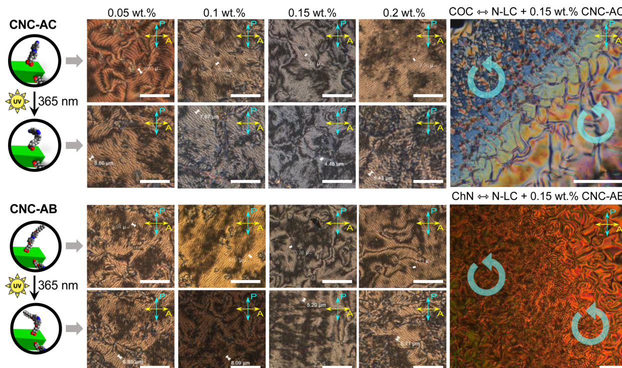
Fig. 3 POM photomicrographs (crossed polarizer, P, and analyzer, A) taken on cooling from the isotropic liquid phase at a T of 45 °C, showing the fingerprint textures obtained from the samples prepared between two untreated glass slides of Felix-2900-03 doped with CNC-AC or CNC-AB before and after illumination with UV light at a wavelength of \lambda = 365 nm at concentrations of the CNCs ranging from 0.05 to 0.2 wt% as indicated above each column of images. Images on the right of each set show the contact preparations with cholesteryl oleyl carbonate (COC) for CNC-AC (taken at T = 45 °C on cooling) or cholesteryl nonanoate (ChN) for CNC-AB (taken at T = 65 °C on cooling), and in each case, no discontinuation was seen in contact with the two known left-handed N*-LCs (handedness is indicated by light blue circular arrows). Scale bars = 50 \mu\text{m} .
