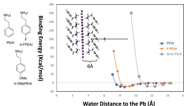
Fig. 14 Plots for theoretically calculated binding energy vs. water distance from the Pb layer for the RP-perovskites based on PEA, 4-FPEAI, and 4-OMePEAI spacers. 64 Reproduced with permission from ref. 64. Copyright 2019, John Wiley and Sons.
