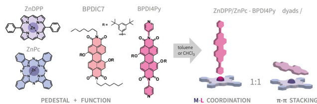
Fig. 1 General scheme of dyad design and components: (left to right) ZnPc and ZnDPP molecular pedestals, the perylene-functional components BPDIC7 and BPDl4Py, and the resulting dyad and triads obtained via metal–ligand (M–L) or \pi – \pi associations in a 1 : 1 or 2 : 1 ratio.
