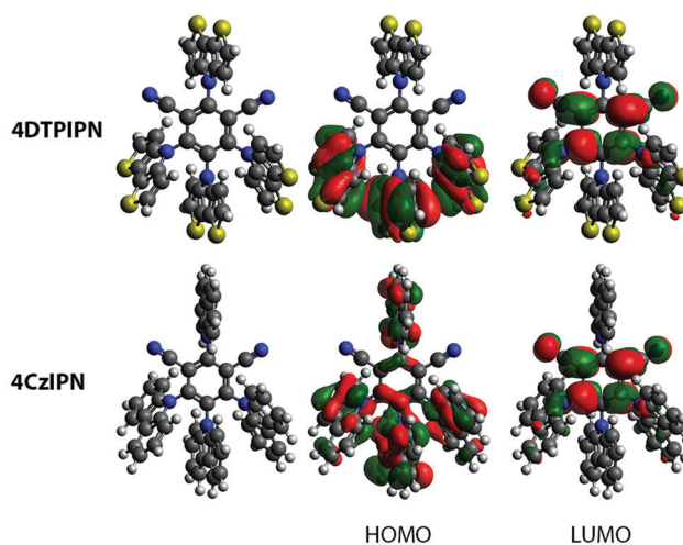
Fig. 1 Optimized geometries and HOMO and LUMO for 4DTPIP and 4CzIPN . Isosurface values of 0.02 a.u. were used for all orbitals.
