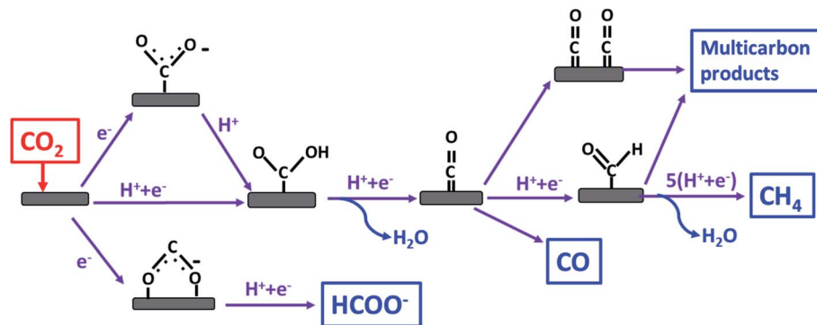
Fig. 1 Scheme of the CO 2 reduction pathway toward different reaction products.
