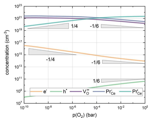
Fig. 7 Calculated defect concentrations of LSF and PCO at 600 °C between 10^{-10} and 1 bar p(\text{O}_2) , calculated from literature data. 62,64,65
