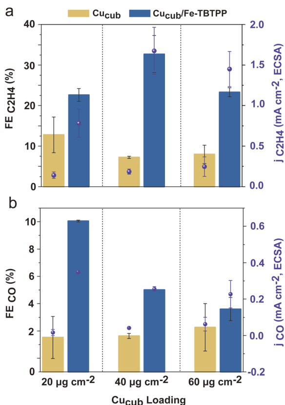
Fig. 7 (a) FE and partial current density for the C 2 H 4 product normalized by ECSA ( j_{\text{C}_2\text{H}_4, \text{ECSA}} ) and (b) FE and partial current density for the CO product normalized by ECSA ( j_{\text{CO}, \text{ECSA}} ) for Cu cub /Fe-TBTTP at different loading of Cu cub ( 3.12 \times 10^2 , 6.24 \times 10^2 and 9.36 \times 10^2 nmol cm -2 ) with the same Fe-TBTTP loading (16 nmol cm -2 ) at -0.95 V vs. RHE in the CO 2 saturated 0.1 M KHCO 3 H-cell. The reported values are an average of three independent experiments with error bars indicating the standard deviations.
