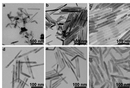
Fig. 2 TEM images of \text{CoF}_2 nanorods: (a) 20 min, (b) 40 min, and (c) 60 min. TEM images of products obtained by injecting solution B (containing different amounts of Li(TFA)) into solution A: (d) 0.05 mmol, (e) 0.01 mmol, and (f) 0.1 mmol.
