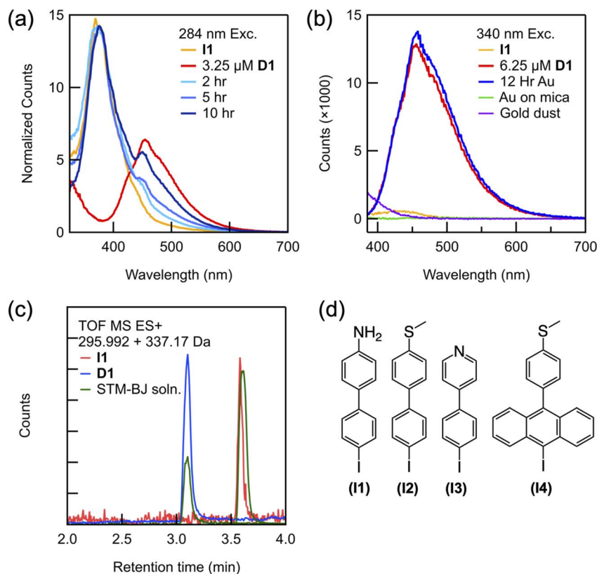
Fig. 2 (a) Emission spectra ( \lambda_{\text{ex}} = 284 \text{ nm} ) of a solution of I1 placed on a rough Au-coated steel substrate over time (blue traces) overlaid with reference peaks for I1 (yellow trace) and an ex situ synthesized solution of D1 (red trace). These traces are normalized to have the same peak height at 380 nm. (b) Emission spectra ( \lambda_{\text{ex}} = 340 \text{ nm} ) showing a peak for D1 that appears in solution left on a rough Au-coated steel substrate (blue trace) overlaid with reference peaks for I1 (yellow trace) and D1 (red trace). Also shown are data from a solution is left on a smooth Au-coated mica substrate (green trace) and with an added suspension of Au dust (purple trace). (c) Selected ion chromatogram (LC-MS) of the I1 standard (red), the D1 standard (blue), and the solution subject to STM-BJ measurements for 12 hours (green). Masses obtained from these spectra are noted in the legend and shown in ESI Fig. S4.† (d) Molecular structures of aryl iodides studied here I1 – I4 .
