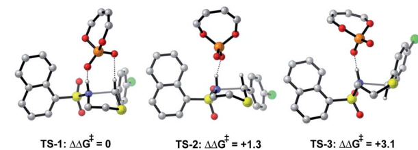
Fig. 2 DFT calculations at the M06-2X/6-31(d,p)//B3LYP/6-31G(d,p) level with the model catalyst system suggest Mechanism B to be operational. All energies quoted in kcal mol -1 .
