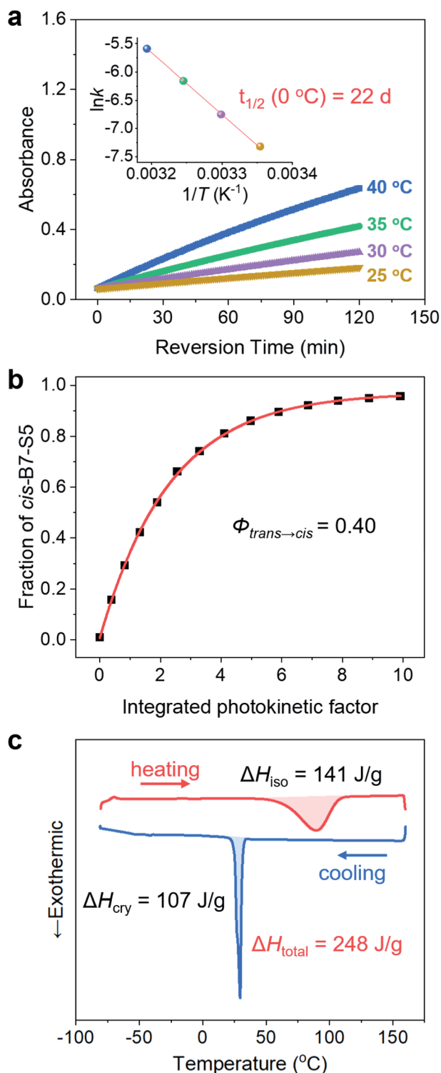
Fig. 4 (a) Thermal cis-trans recovery of cis -B7-S5 in acetonitrile with time at different temperatures followed by the absorbance increase at \lambda_{\max} = 385 nm. The inset shows the linear fit between \ln k and 1/T according to the Arrhenius equation. (b) Exponential fitting of the fractions of cis -B7-S5 against the integrated photokinetic factor x(t) . (c) First heating (red) and subsequent cooling DSC curves (blue) of cis -B7-S5.
