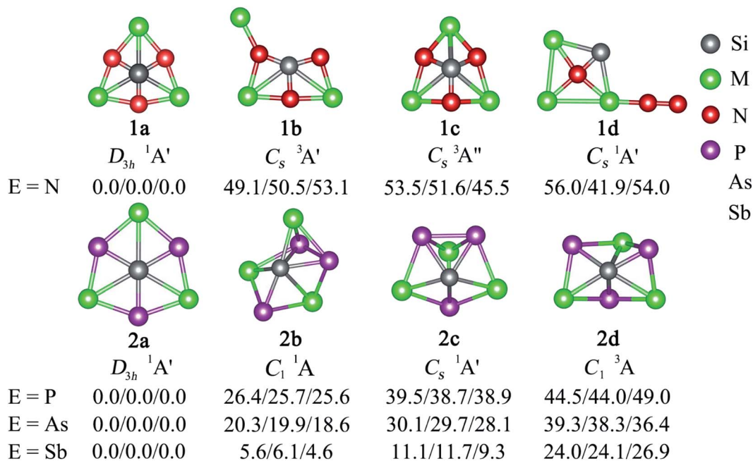
Fig. 2 The structures of low-lying isomers of \text{SiE}_3\text{M}_3^+ ( E = \text{N, P, As, Sb} ; M = \text{Ca, Sr, Ba} ) clusters. Relative energies (in kcal mol -1 ) are shown at the single-point CCSD(T)/def2-TZVP//PBE0/def2-TZVP level, followed by a zero-energy correction at PBE0. The values from left to right refer to Ca, Sr, and Ba in sequence. The group symmetries and electronic states are also given.
