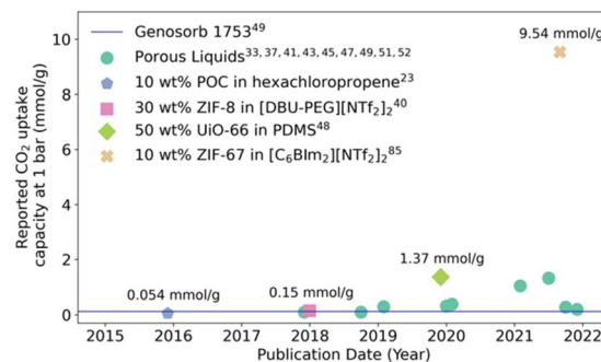
Fig. 5 Reported \text{CO}_2 uptake capacities in porous liquids at ca. 1 bar and ca. 298 K over time. A selection of the significant developments are highlighted to show the acceleration in progress.
