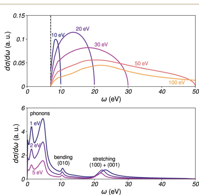
Fig. 4 Singly-differential cross sections for inelastic scattering. Top: SDCS for electronically inelastic events, for incident kinetic energies E = 10, 20, 30, 50 and 100 eV. The black vertical line marks the excitation threshold for liquid water. Bottom: SDCS for vibrationally inelastic events, for E = 1, 2 and 5 eV.
